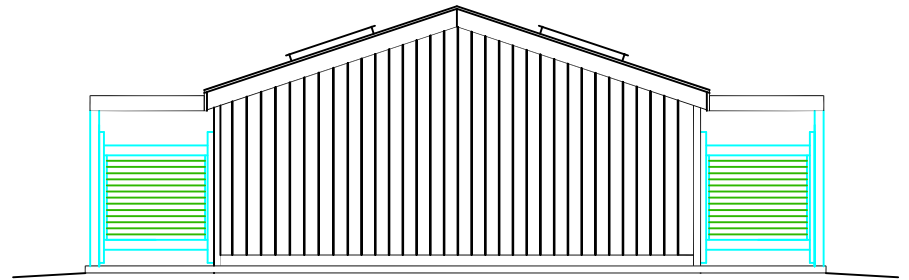
FRONT ELEV.
