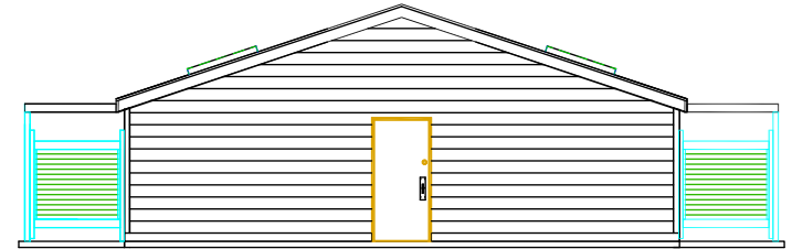
END ELEVATION @ CHASE DOOR
