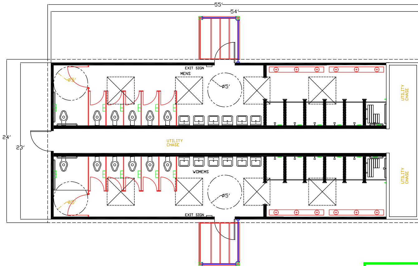
FLOOR PLAN
