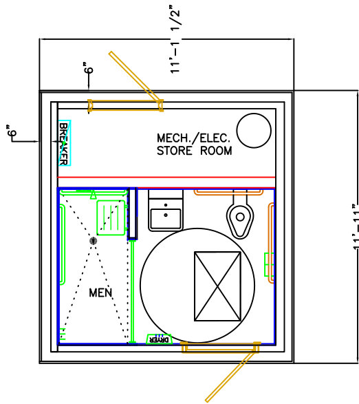
FLOOR PLAN
