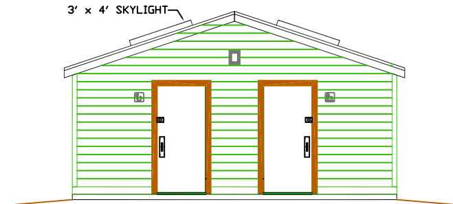
FRONT ELEVATION OPTIONAL ROOF PACKAGE (REV)
