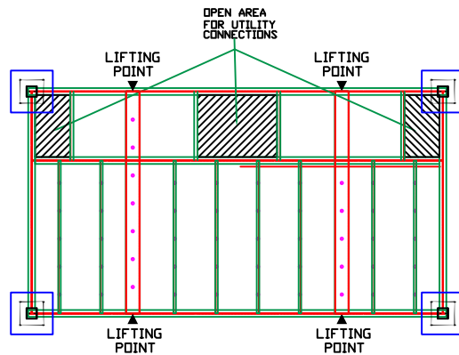
PIER LOCATION PLAN STEEL FRAMING & LIFTING
