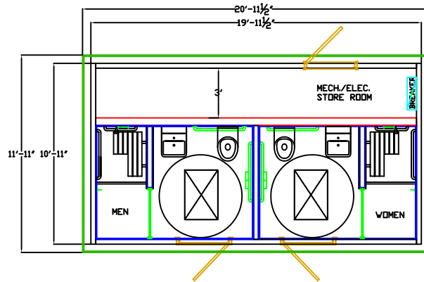
FLOOR PLAN
